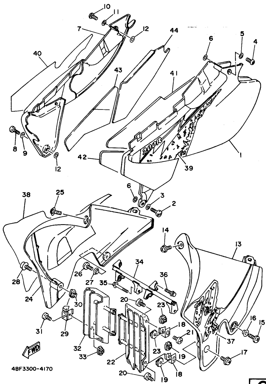
FIG. 17 SIDE COVER
