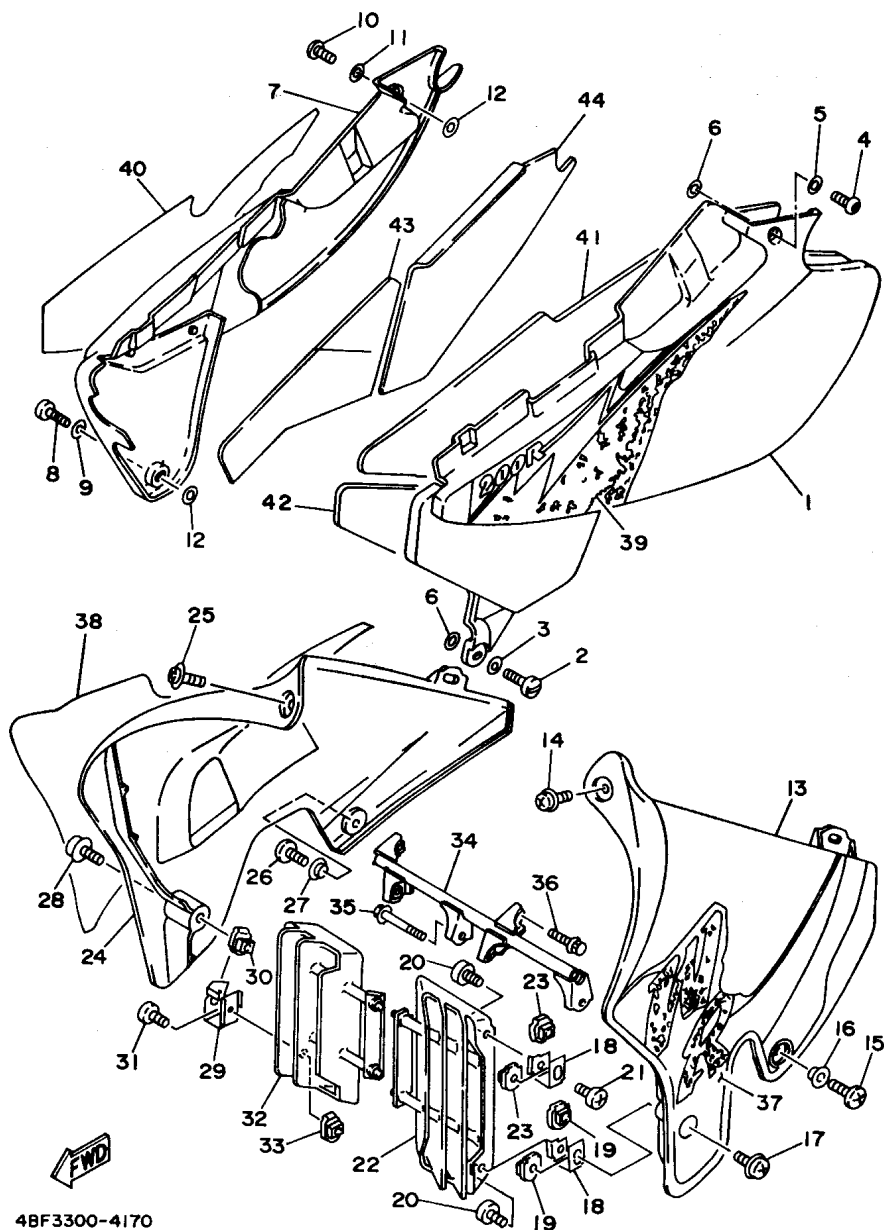
FIG. 17 SIDE COVER
